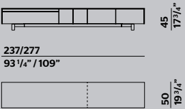
FLOOR STANDING BASES WITH METAL BASE BASI A TERRA CON BASAMENTO
