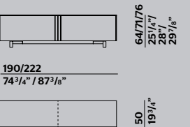
FLOOR STANDING STORAGE UNITS WITH FLUSH SLIDING DOORS AND METAL BASE CONTENITORI COMPLANARI A TERRA CON BASAMENTO
