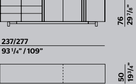
FLOOR STANDING SIDEBOARD WITH METAL BASE MADIE A TERRA CON BASAMENTO
