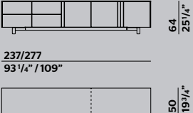
FLOOR STANDING STORAGE UNITS WITH METAL BASE CONTENITORI A TERRA CON BASAMENTO
